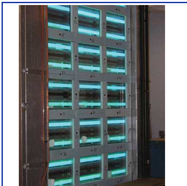
A simulation of weather cycling from hot to cold extremes with moisture added provides accelerated weather cycling testing under the standard.
