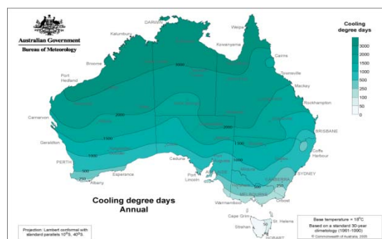
Figure 9-Australian CDD-Cooling Degree Days
